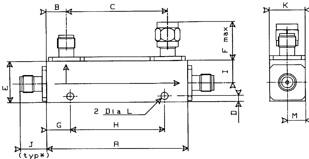
3 SMA/f connectors
